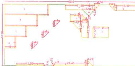
AREA CALCULATION OF EXISTING MODIFIED SECOND FLOOR PLAN BUILDING - B SCALE 1:100
