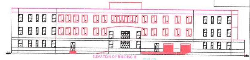
ELEVATION OF BUILDING B SCALE 1:100
